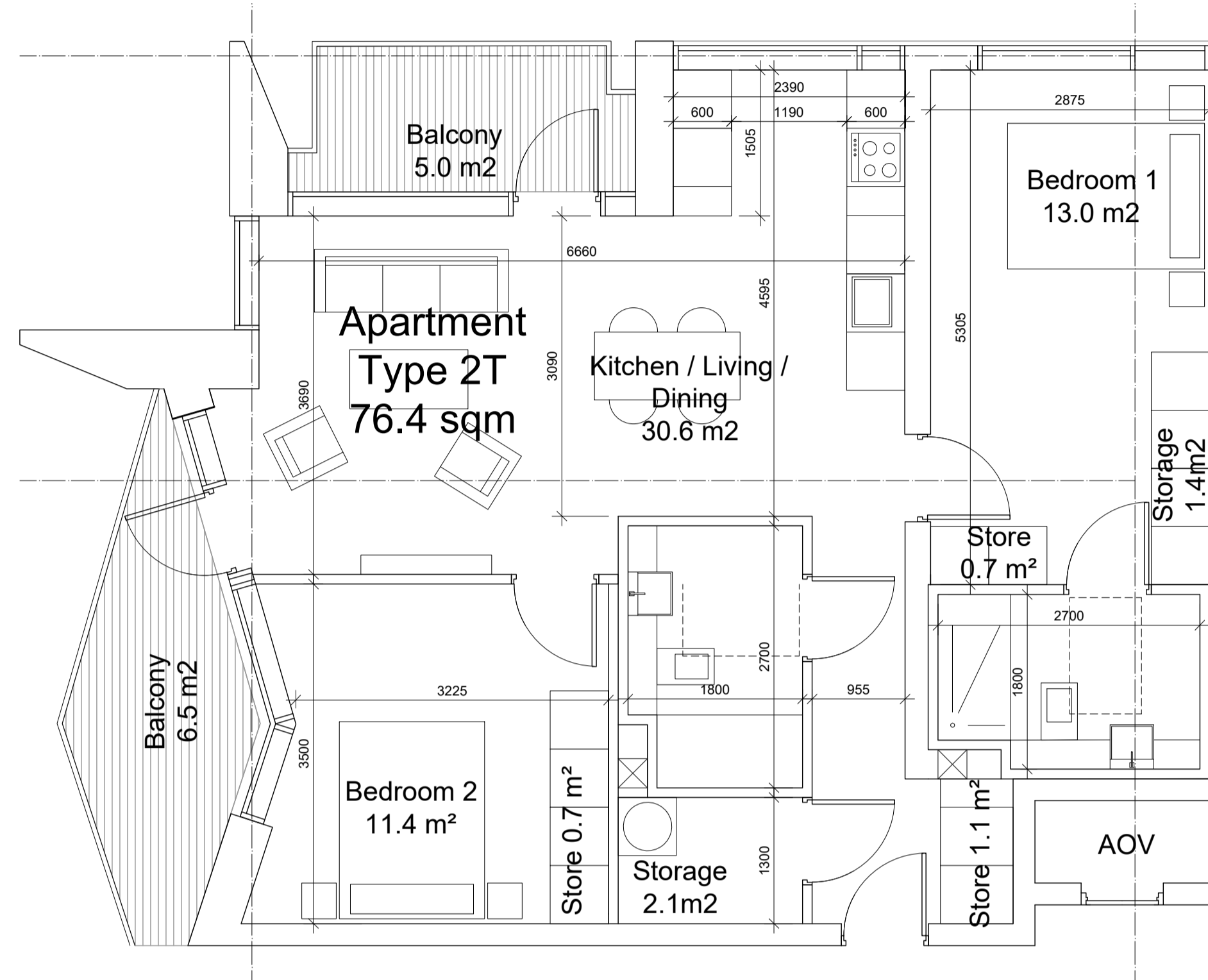
01 PL1927 2 Bed Apartment - Type 2T (1 Unit) SCALE 1:50
