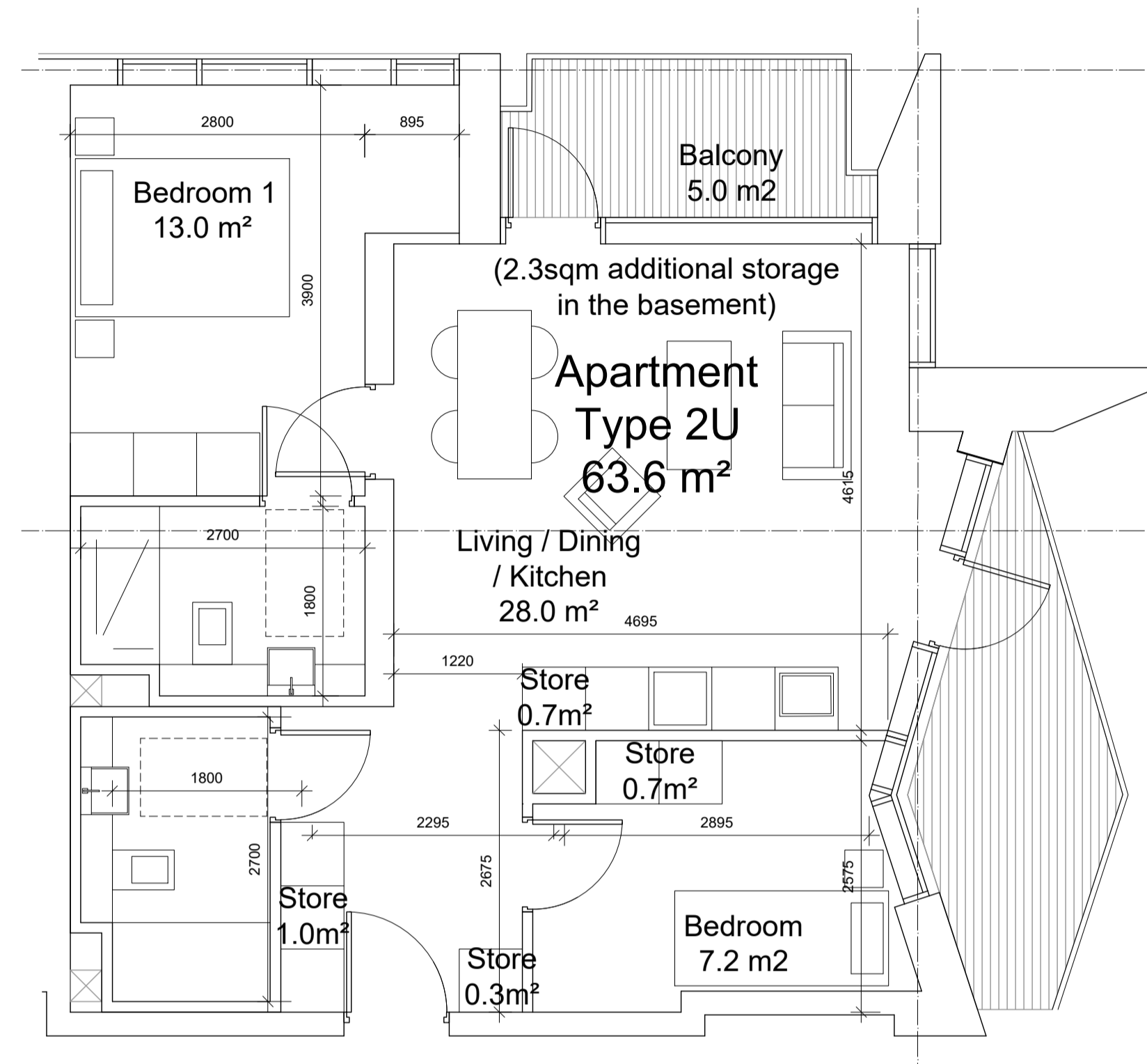
02 PL1927 2 Bed Apartment - Type 2U (1 Units) SCALE 1:50
