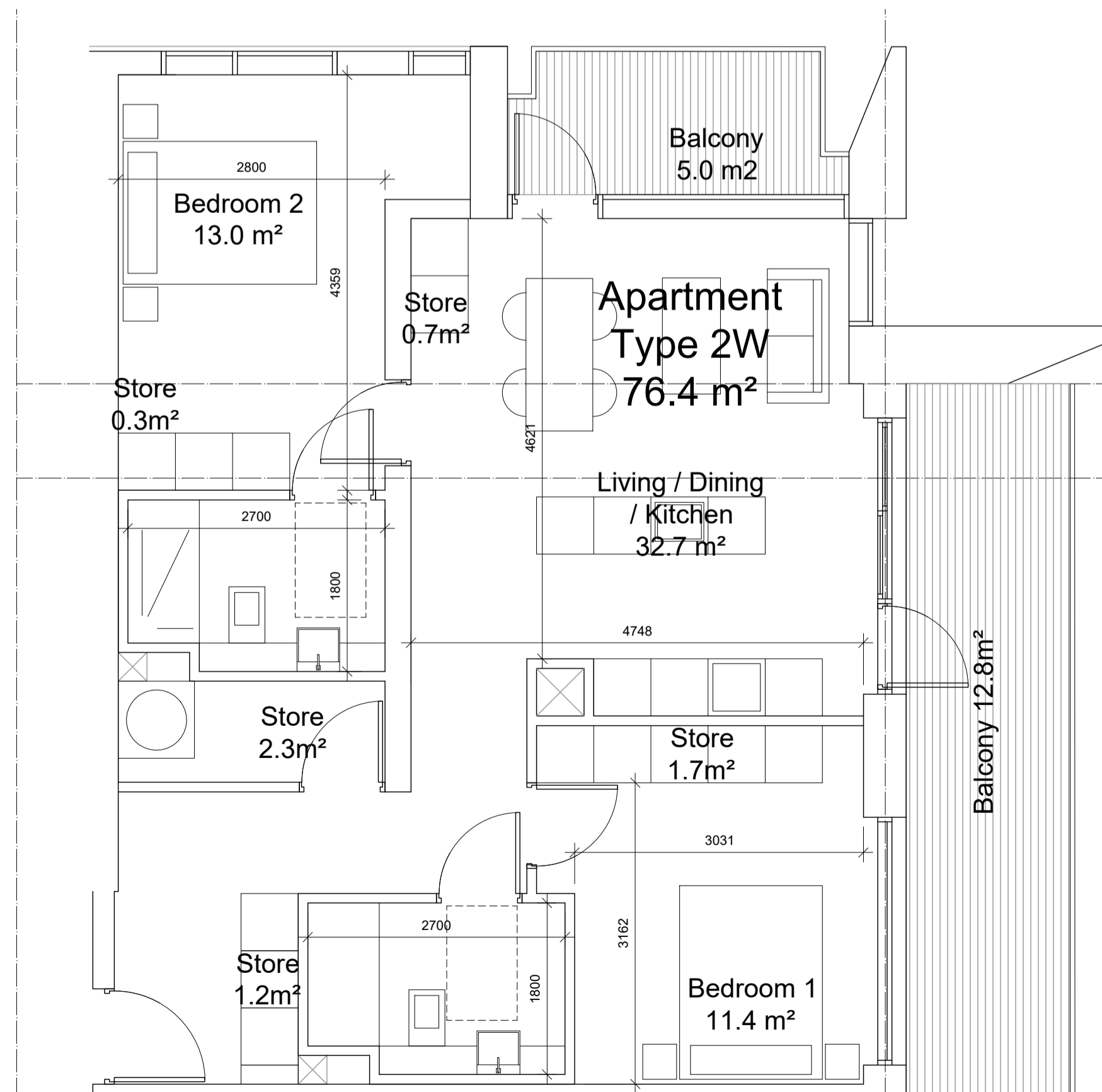
04 PL1927 2 Bed Apartment - Type 2W (1 Units) SCALE 1:50
