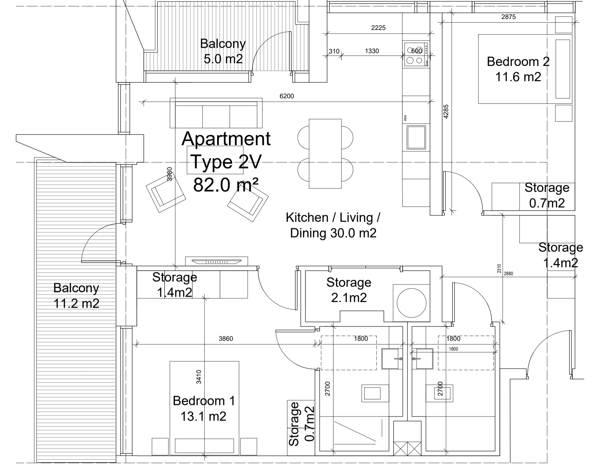
03 PL1927 2 Bed Apartment - Type 2V (2 Units) SCALE 1:50
